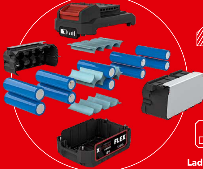
Accu-machine
